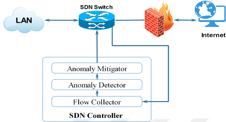
Figure 2.4 NIDS Architecture in the SDN controller
