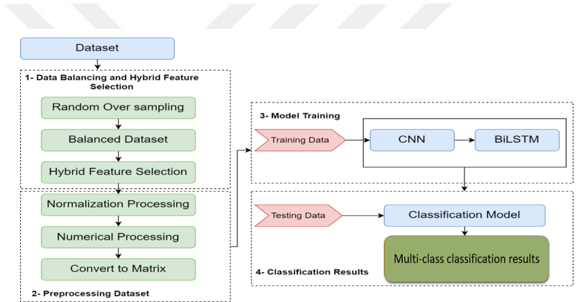
Figure 3.1 Architecture of proposed framework NIDS in SDN
