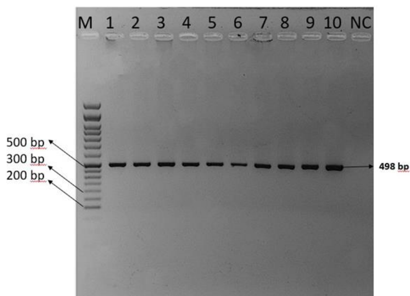
Figure 1. Agarose gel electrophoresis image of PCR products of the OLFML3 gene. (M: Marker, Column 1-10: 498bp PCR product, NC: Negative Control)
